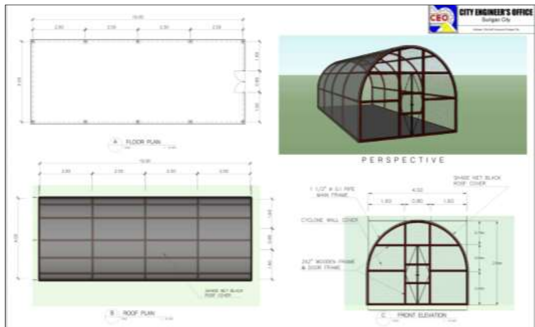
Figure 1. Sample perspective view of the proposed Nursery Shed at Sanitary Landfill
